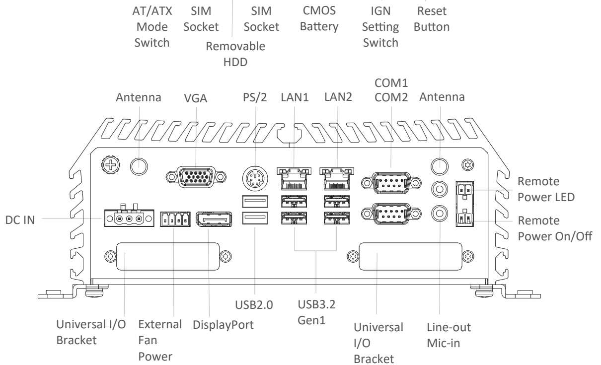
Rear I/O
