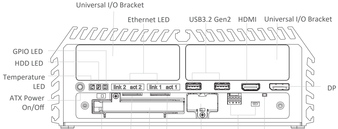
Front I/O
